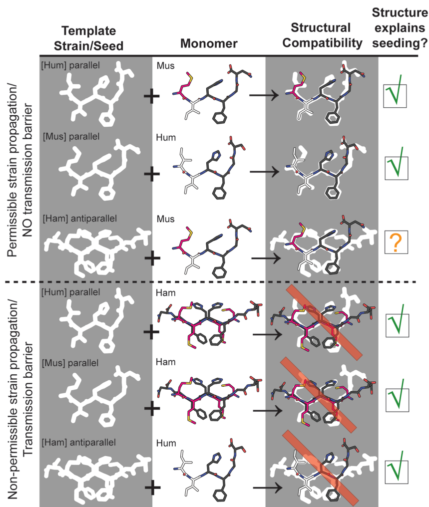
Figure 2. Structural compatibility as a molecular mechanism for permissible prion strain propagation and transmission barriers. The left column represents template strains or seeds as a mold; the middle column represents monomers as sticks. To have successful seeding, the sticks have to fit in the mold. The right column shows the quality of the fit. The fourth column shows how this rationalization of structural fit matches the data presented by Vanik et al. and Jones et al. and summarized in Table 1 for the species-dependent seeding of PrP 23–144 . 25,26
