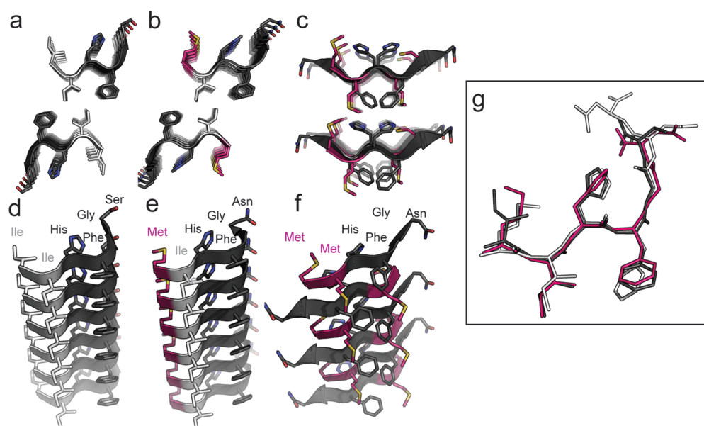
Figure 1. Atomic structures from X-ray crystallography of steric zippers formed by the transmission-determining segment of human, mouse, and hamster PrP. The steric zippers of human (a), mouse (b), and hamster (c) segments 138–143 (using human numbering) are illustrated as cartoon representations showing sheet-to-sheet interactions. Side chains are drawn as stick representations, with carbon atoms in isoleucine residues highlighted in white, methionines in magenta, and the remaining residues in dark gray. In the side chains, nitrogen atoms are colored in blue, oxygen in dark red, and sulfur in yellow. The bottom panels (d–f) show a view perpendicular to the hydrogen-bonding axis (length of the page) of one isolated sheet showing the stacking of \beta -strands. By comparing panels a and b it can be seen that the two structures of human and mouse segments and interfaces are nearly identical. (g) The alignments of six-residue Hum138–143 (dark gray), six-residue Mus137–142 (magenta), and seven-residue Mus137–143 (white) have similar conformations with the characteristic kink at Gly142. A quantitative comparison can be found in Table 3.
