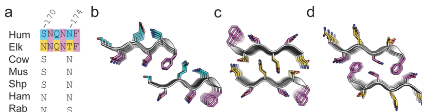
Figure 3. (a) The sequence alignment of the region 170–175 (using human numbering) of human (Hum), elk, hamster (Ham), bovine (Cow), mouse (Mus), sheep (Shp), and rabbit (Rab) PrP. Residues corresponding to positions 170 and 174 using human numbering have species variation; however, only the elk prion has both an Asn at residue 170 and Thr at residue 174. Purple highlights the xNxNxF motif common for all species, while cyan highlights the human-specific residues and yellow highlights the elk-specific residues. These colors are continued in the stick representations of side chains in the human segment 170–175 (b), PDB code 3fva, and both interfaces of the homologous elk segment (c and d), PDB code 2ol9. 22,34 The peptide backbone is depicted as a cartoon in white. In all of the representations the hydrogen-bonding axis of the \beta -sheets is perpendicular to the plane of the page to point out the packing of side chains within the steric zipper interfaces.
